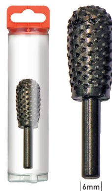
WOOD SEMISPHERICAL ROTARY RASP
